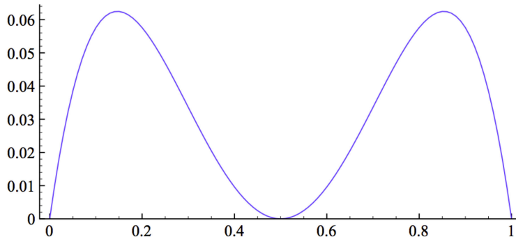
Figure 1: Advantage of playing for a triple as a function of p
